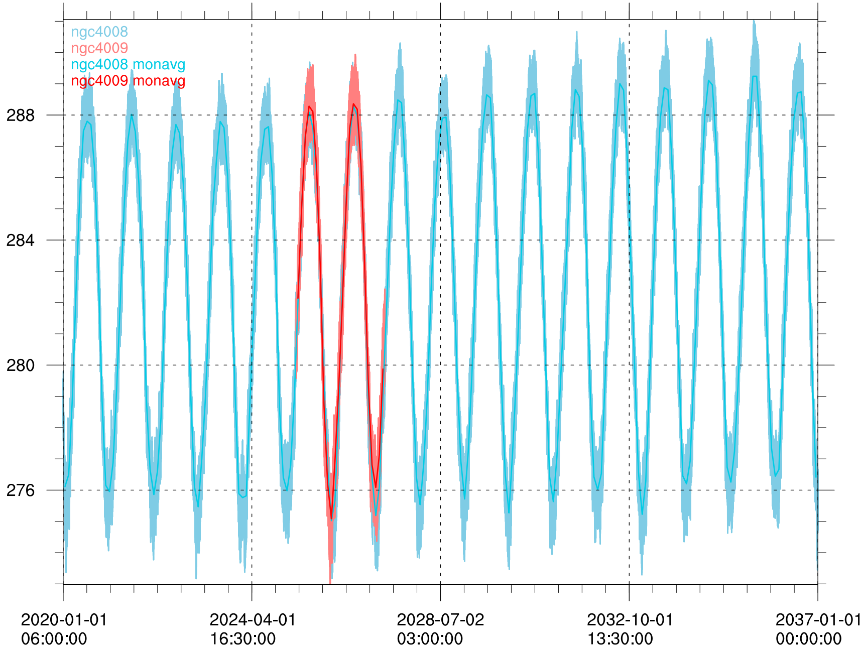
Global land mean surface temperature [K]
