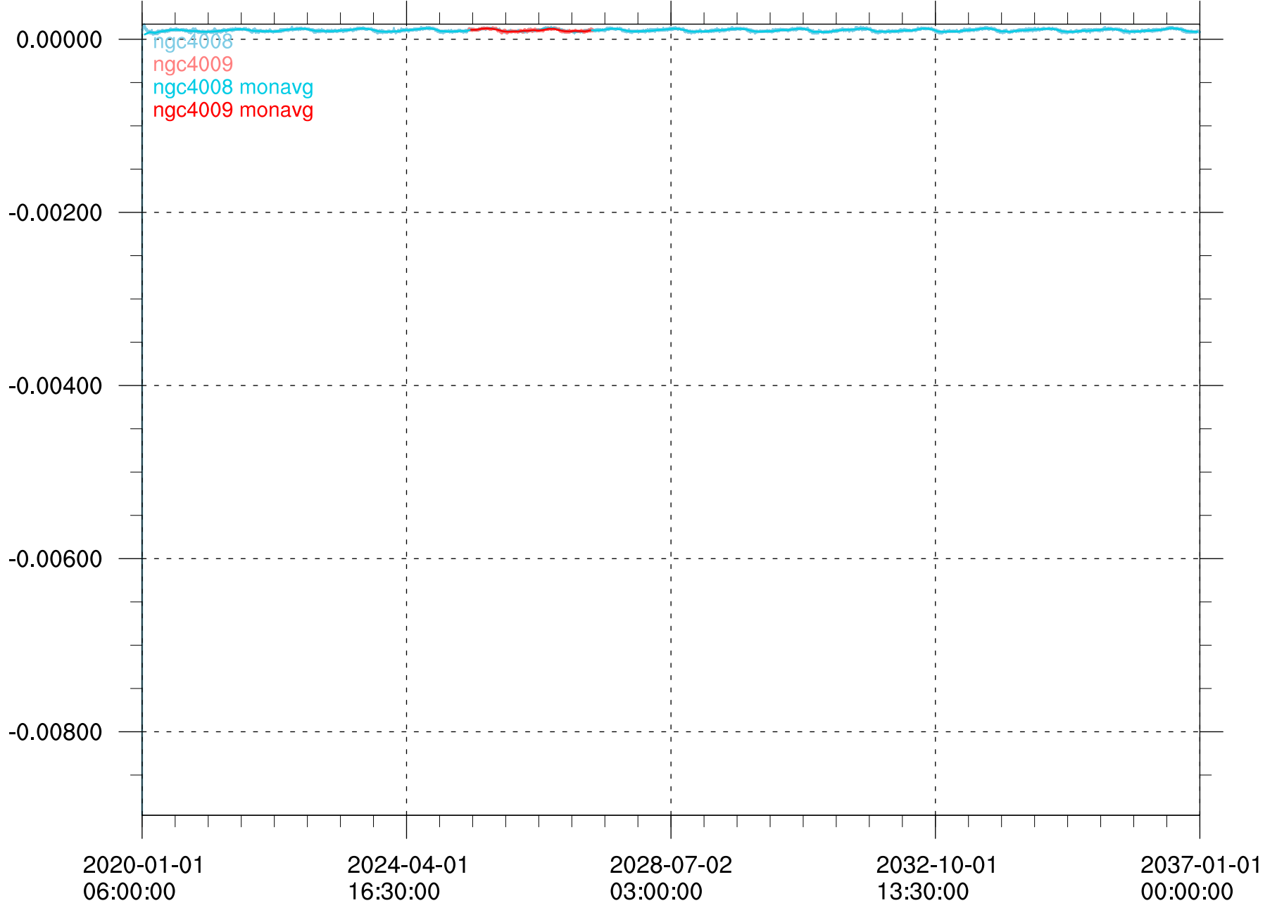
Global land water balance error [m3/timestep]
