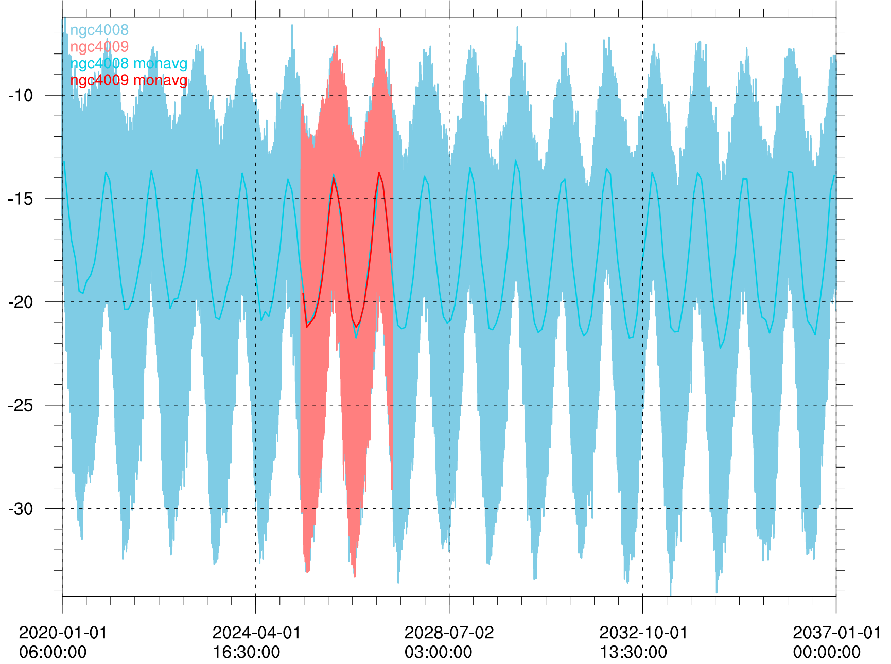
mean energy flux at surface from thermal exchange [W m -2 ]
