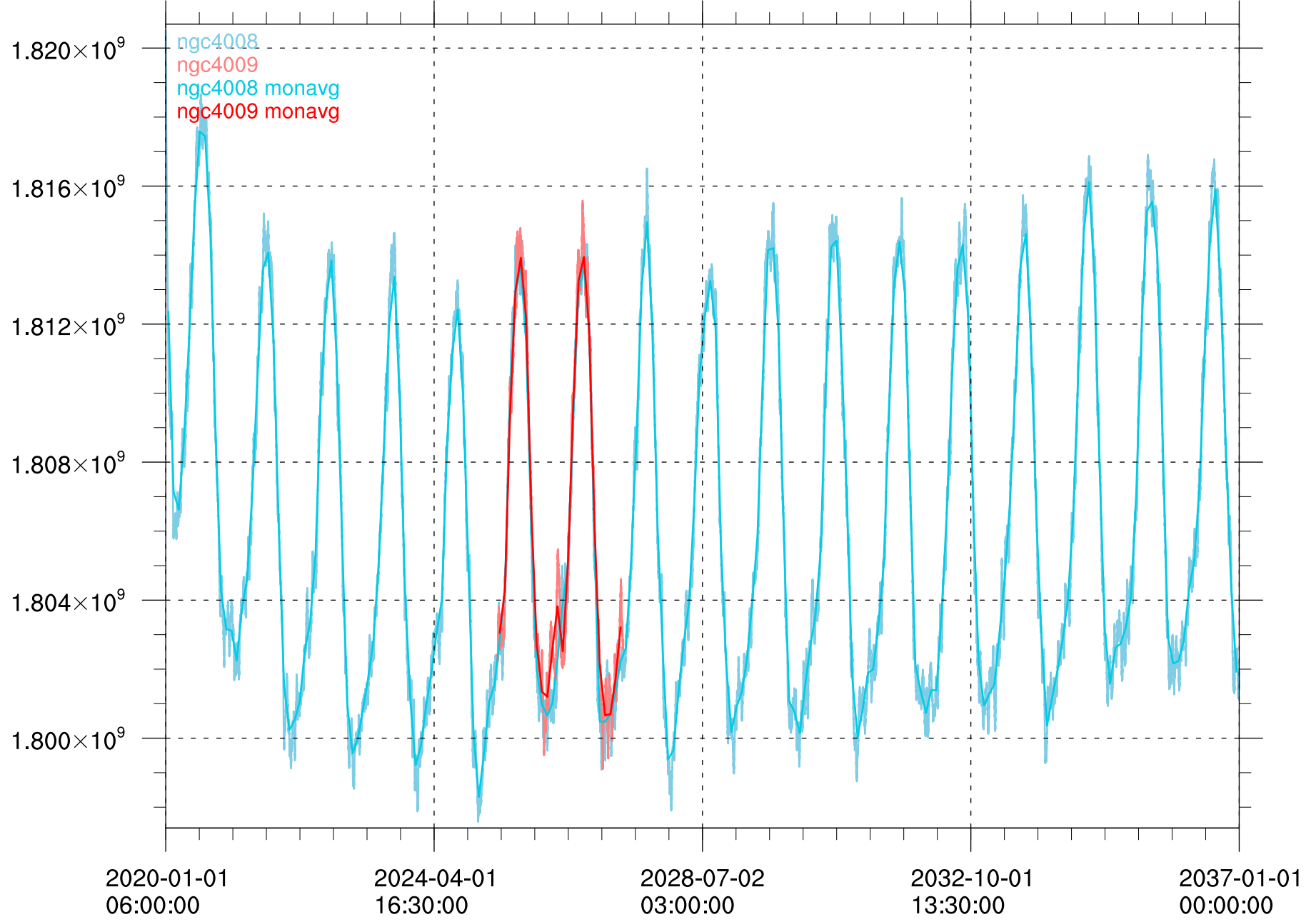
mean vertically integrated moist internal energy after dynamics [J m-2]
