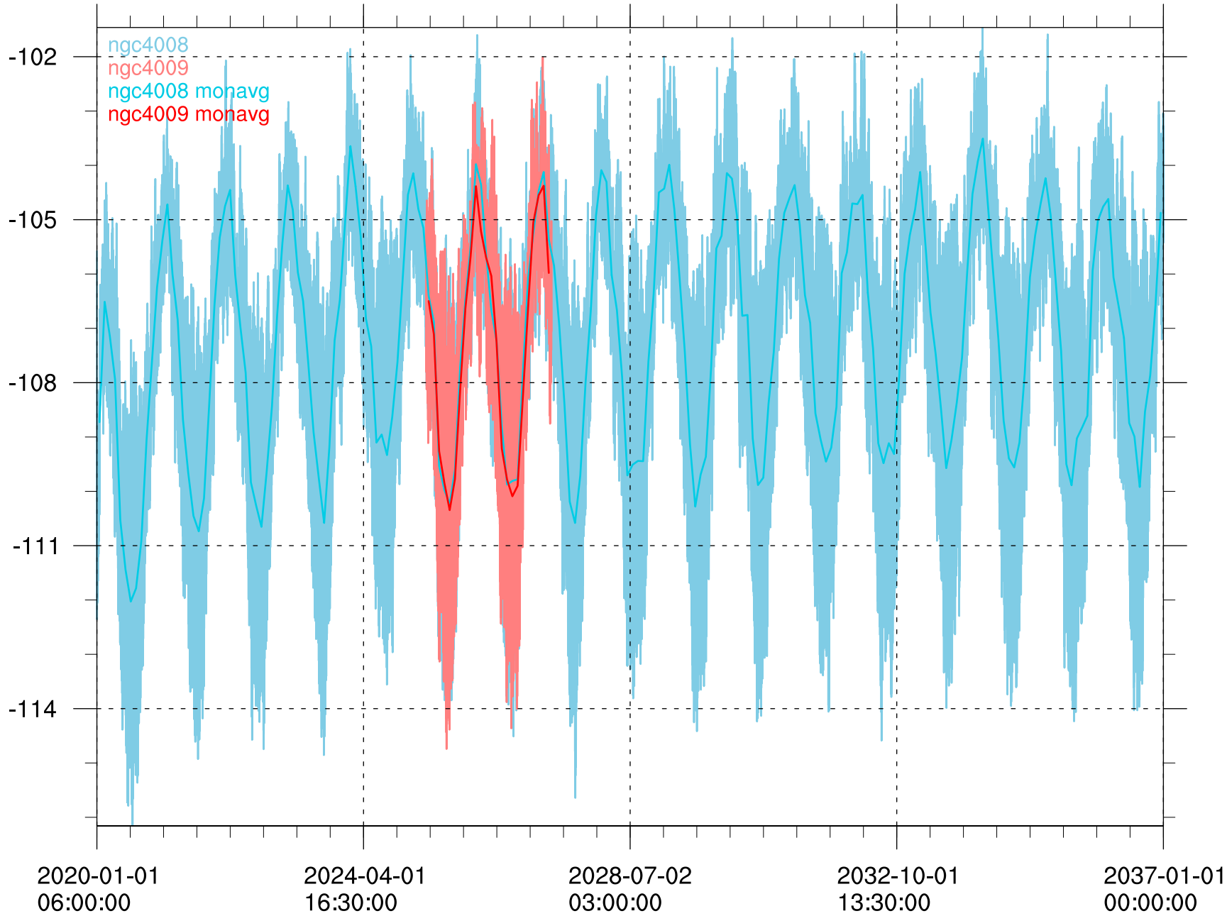
global mean net radiative flux into atmosphere [W m -2 ]
