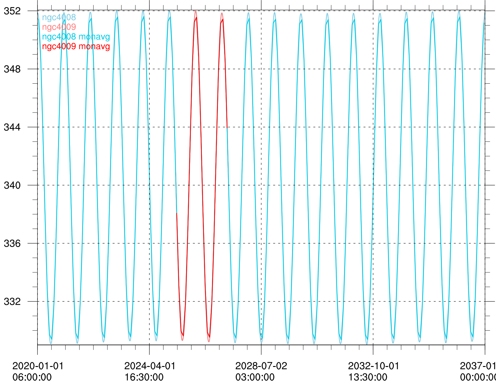
global mean toa incident shortwave radiation [W m-2]
