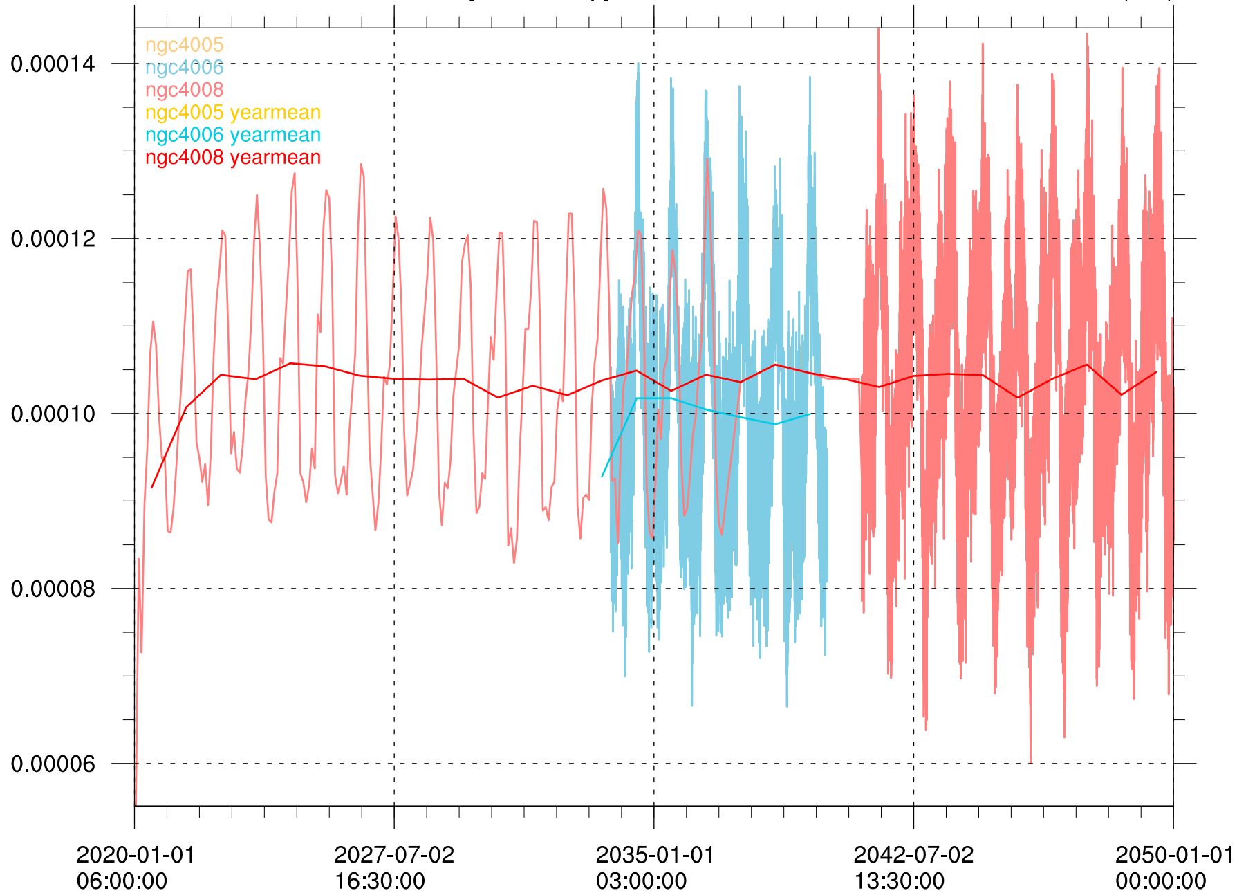
Global land water balance error [m3/timestep]
