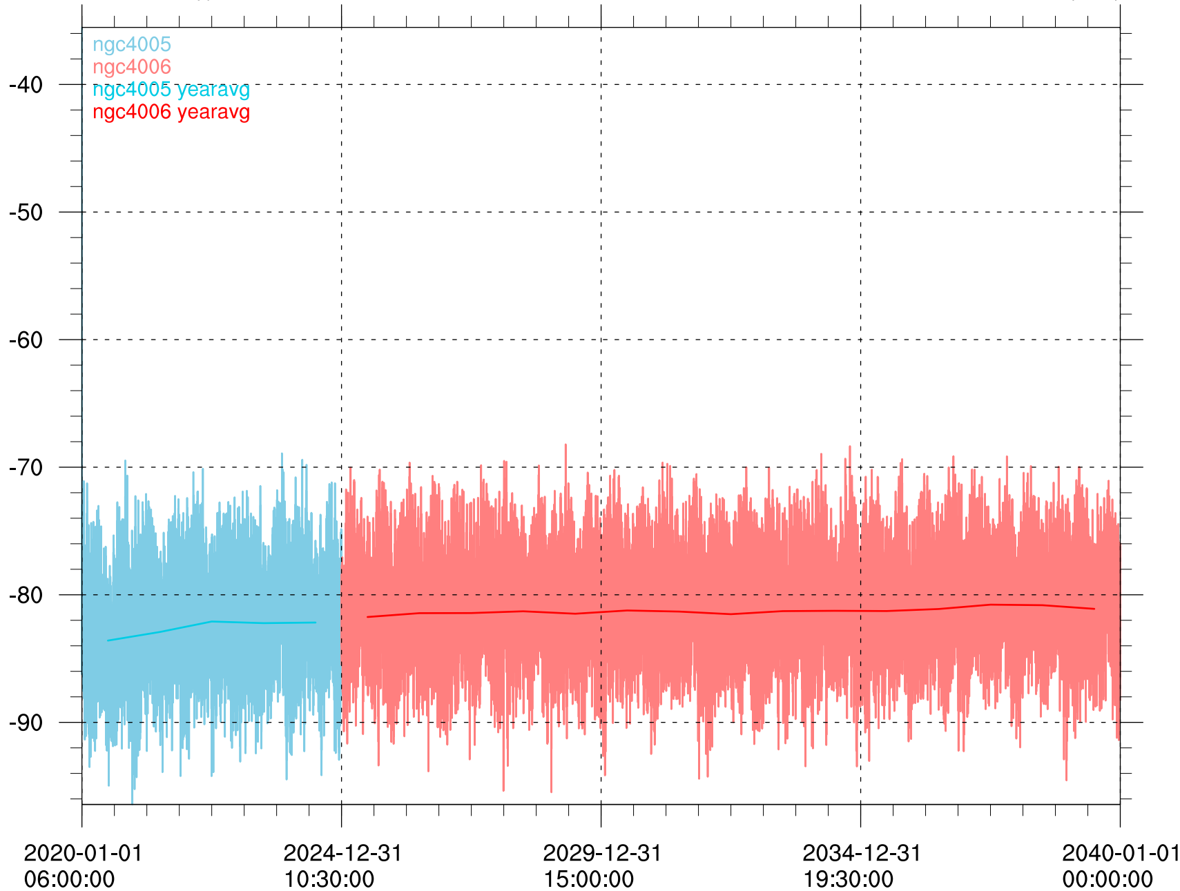
mean energy flux at surface from condensate [W m -2 ]
